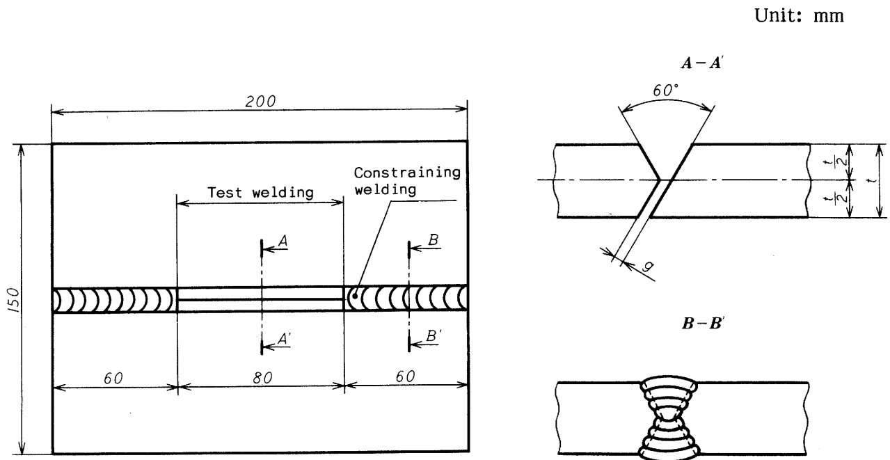
Fig. 1. Shape and dimensions of test plates
