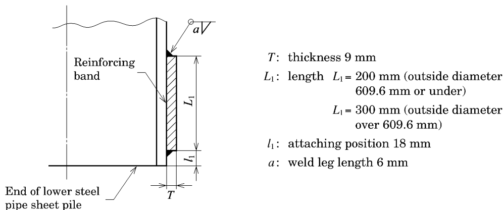
Figure A.1 Example of shape and dimensions of outer surface reinforcing band
